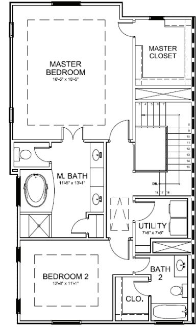
Third Floor
