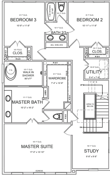
SECOND FLOOR PLAN Scale: 1/4" = 1'-0"
